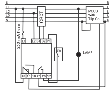
Non Fail Safe Mode with UV Trip Coil
