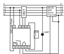
Non Fail Safe Mode with Shunt with Trip Coil
