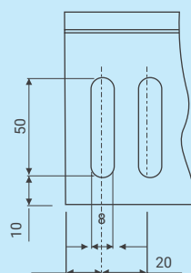
Oblong Slot
