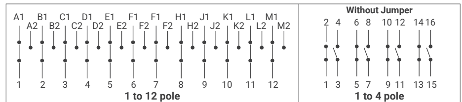
Connection Diagram
