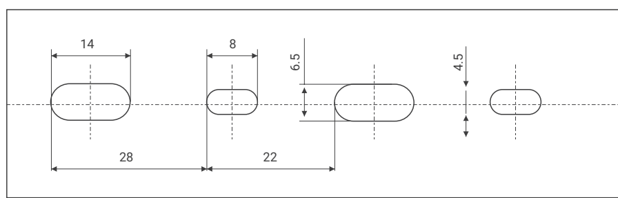
Bottom Mounting Slots for All Sizes
